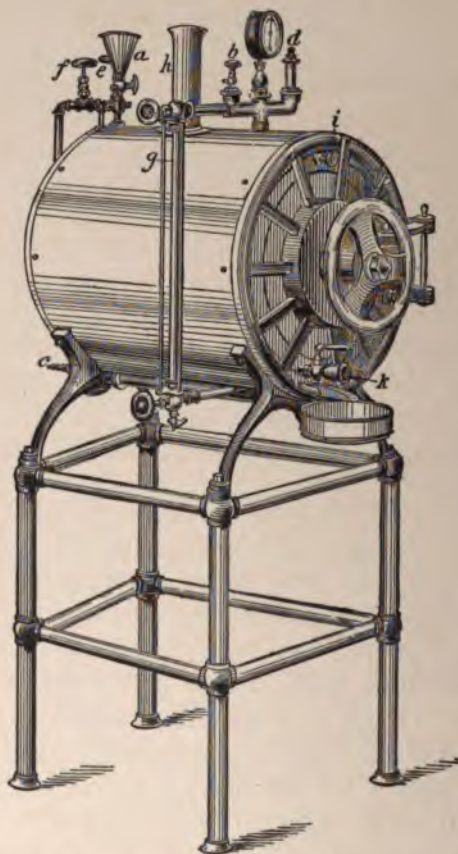
FIG. 42.—Kny-Sprague sterilizer: a , Funnel and valve where water is taken into the jacket; b , valve for discharge of air displaced by the water; c , gas attachment; d , safety-valve; e , valve which controls the steam for vacuum apparatus; f , valve admitting steam from jacket to chamber; g , glass water-gauge; h , ventilating pipe for gas combustion; i , test-valve for steam in chamber; k , air-filtering valve for destroying vacuum.
